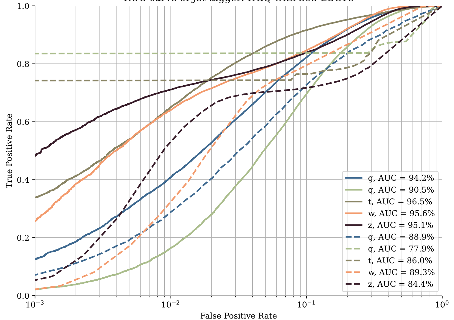
ROC-curve of Jet-tagger: HGQ with 303 EBOPs
